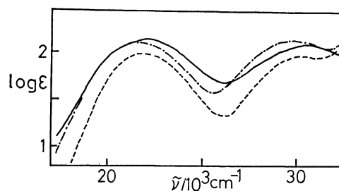
Fig. 2. Absorption spectra of [Co(CN)(Hten)] 3+ (—), and the two isomers of [Co(CN)(Httn)] 3+ , (A) (---) and (B) (-.-).
